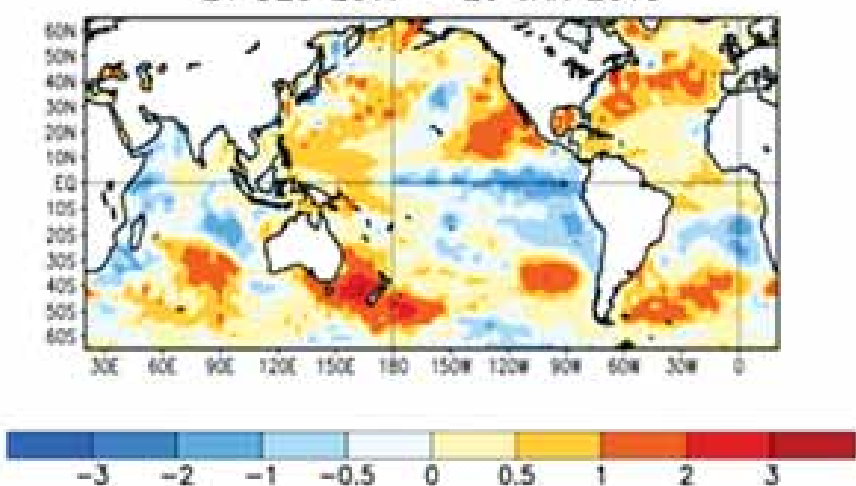
Average SST Anomalies 24 DEC 2017 – 20 JAN 2018
